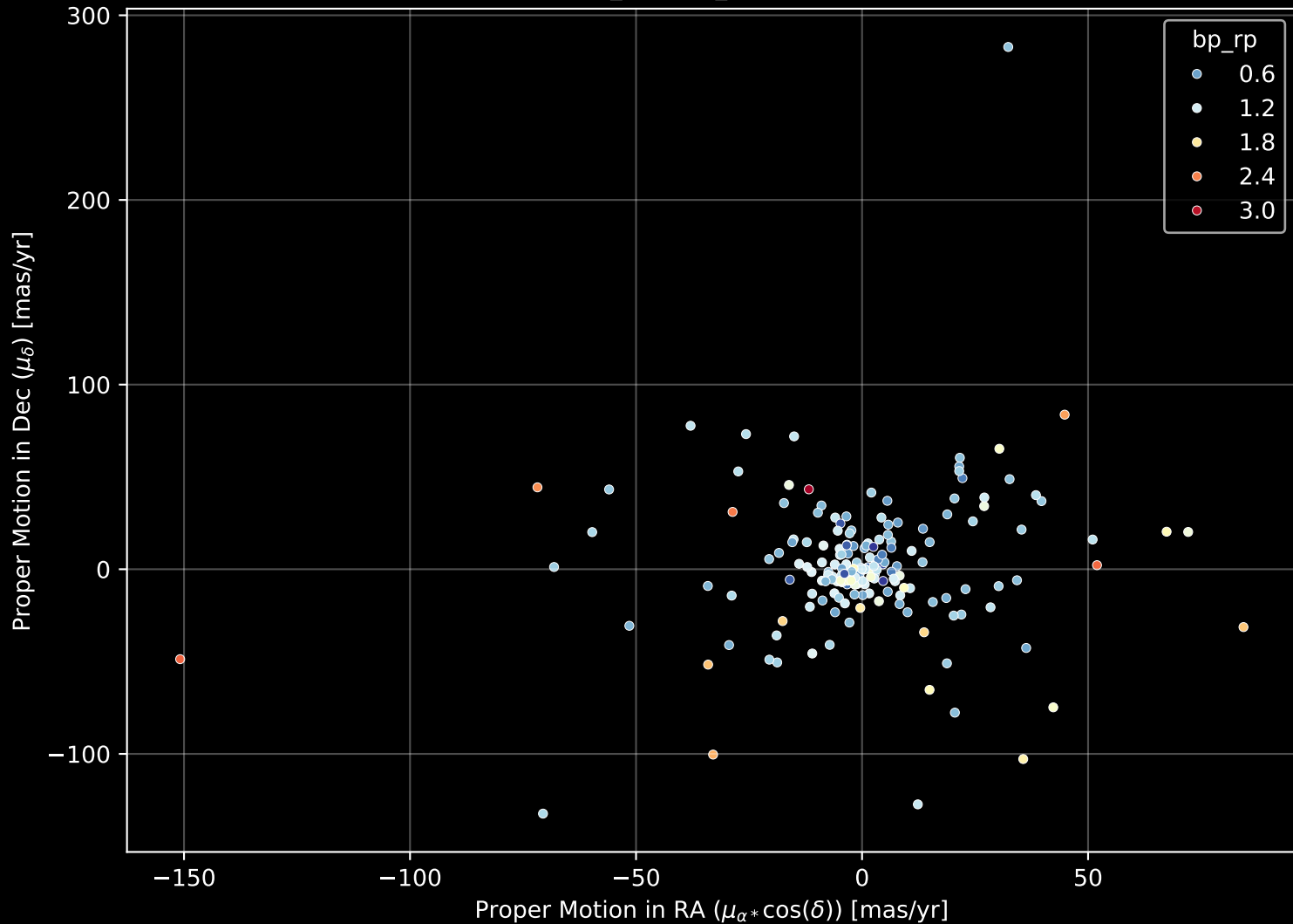
APOGEE DR17 Field: [CVZTILE_088+24_btx] Proper Motion Diagram (n= 185)
