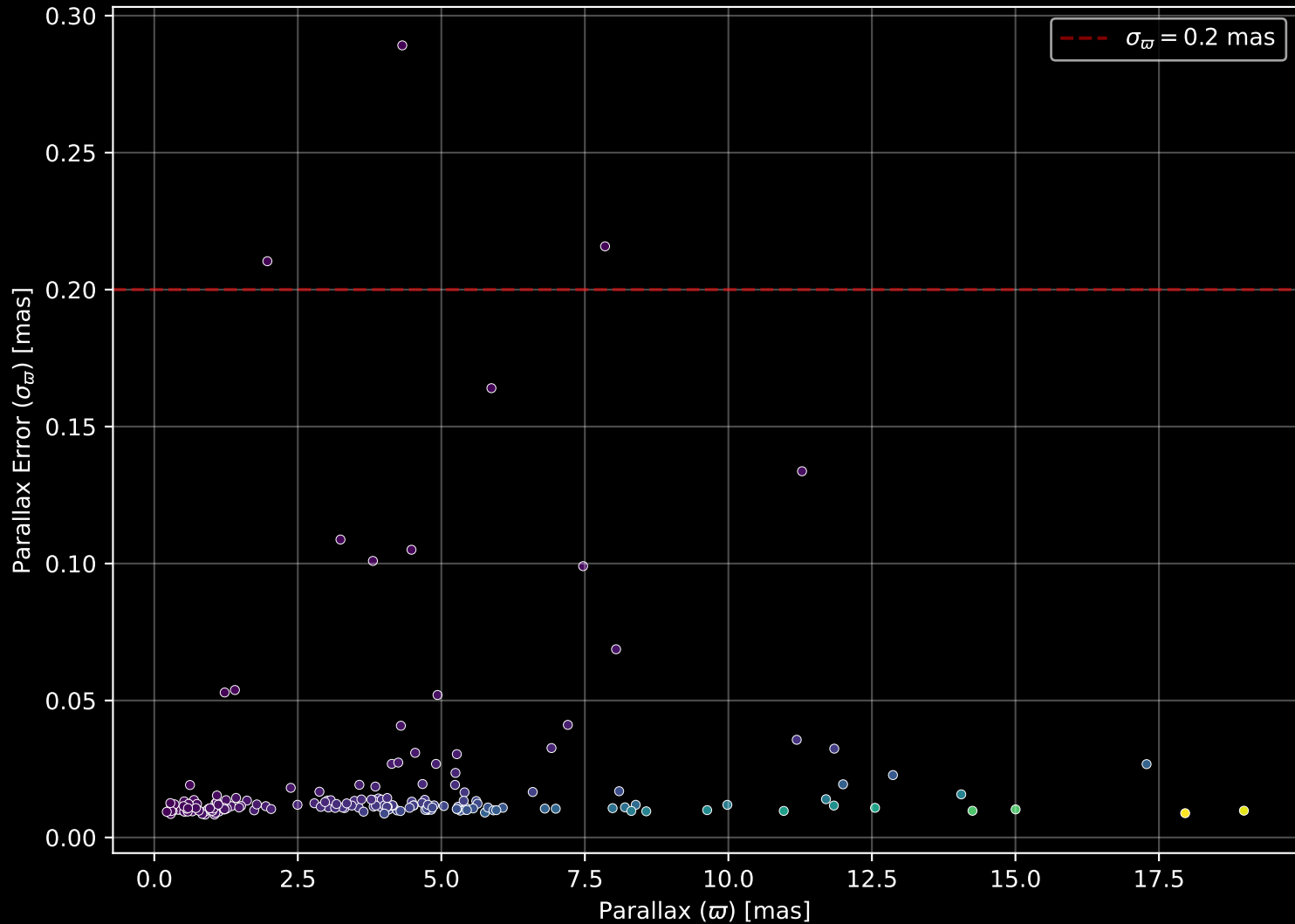
APOGEE DR17 Field: [CVZTILE_088+24_btx] Parallax Quality (n= 185)
