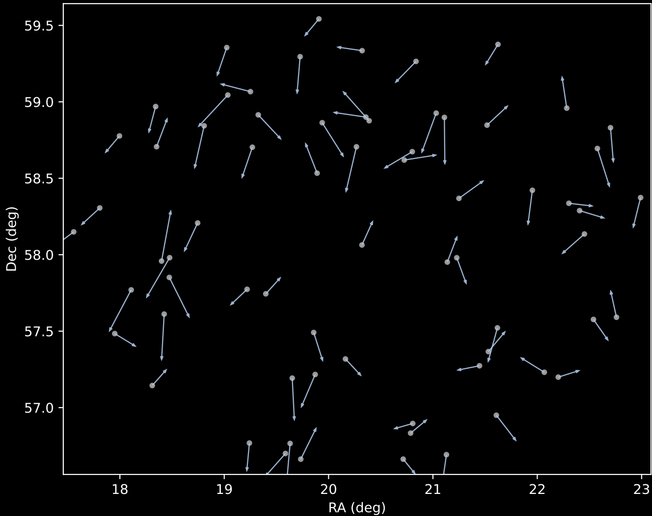
APOGEE DR17 Cluster 1 Proper Motion Vectors (n=68)
