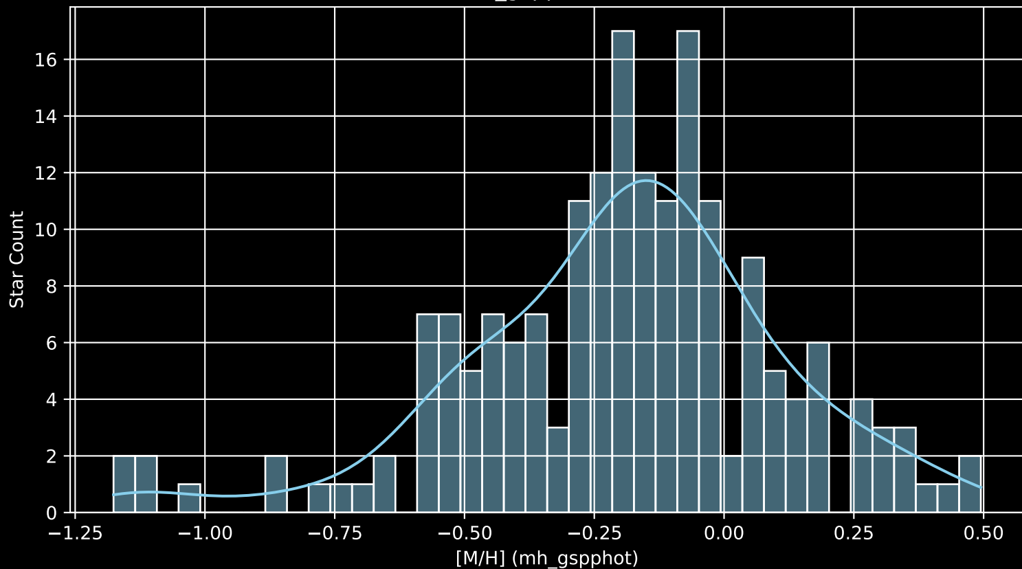
APOGEE DR17 Field: [CVZTILE_088+24_btx [M/H] (mh_gspphot) (n= 185)
