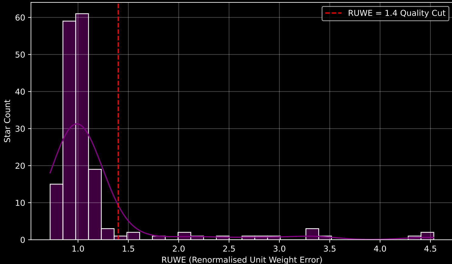
GAPOGEE DR17 Field [CVZTILE_088+24_btx] RUWE Distribution (n= 175)
