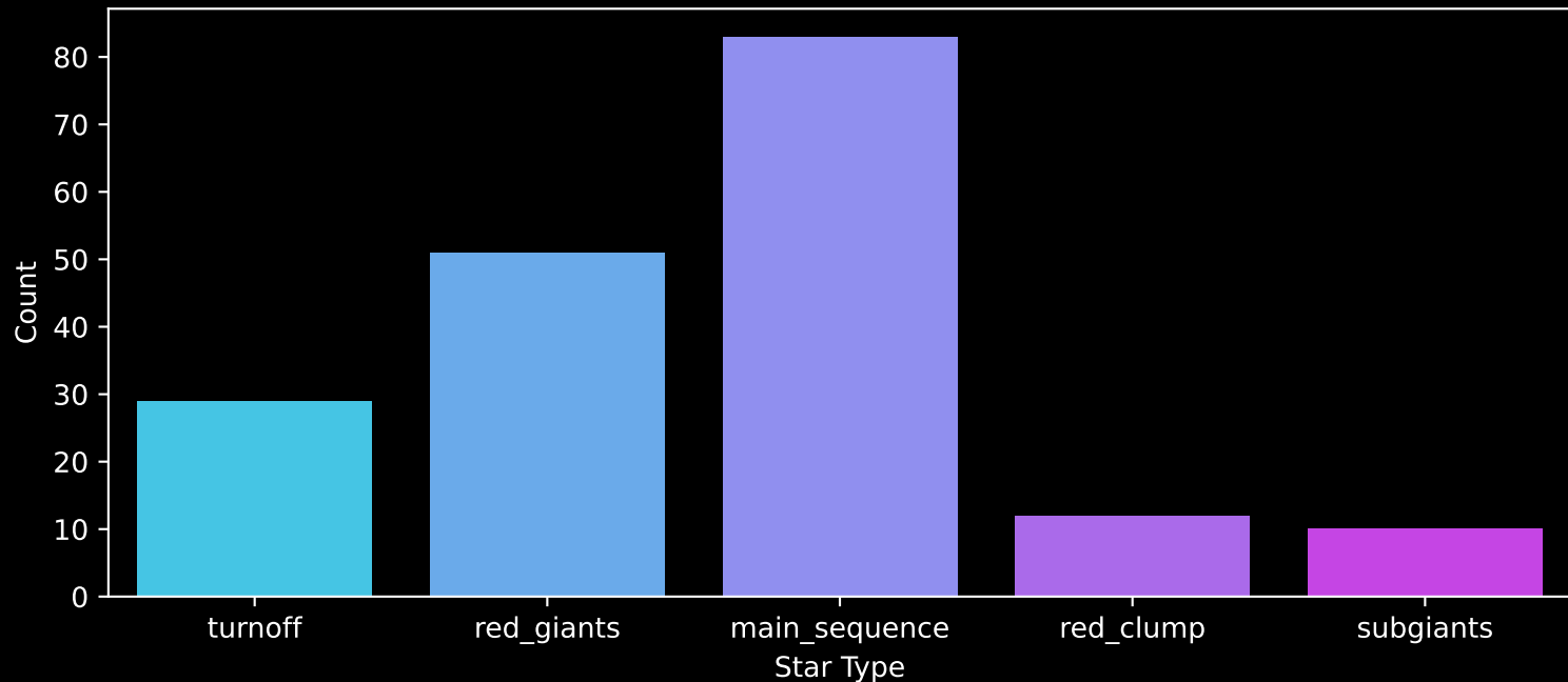
APOGEE DR17 Field: [CVZTILE_088+24_btx] Count plot of Star Type
